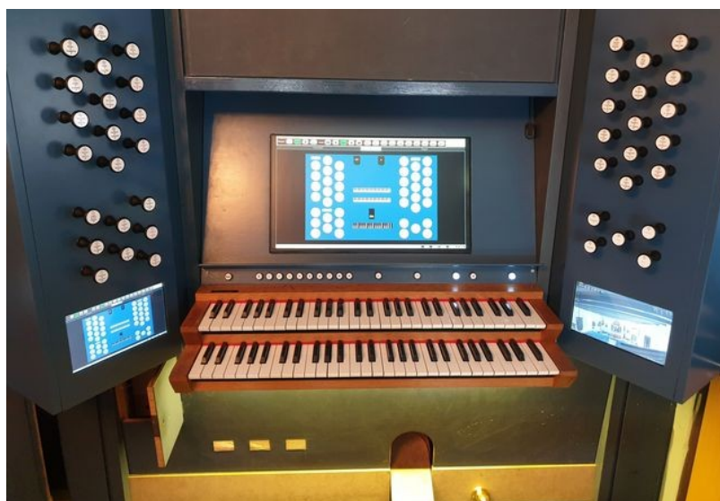
Hornbæk church, Sjælland * expansion from 12 to 36 registers Built with Danhild digital music viewer, digital register control, camera and monitors
